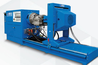
450E Series Transmission Test Stand
