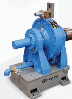
50X Series Water brake engine dynamometer
